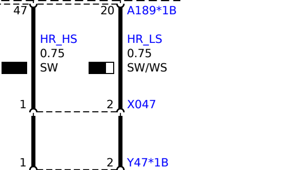
Y47 Valve coil, rear right
