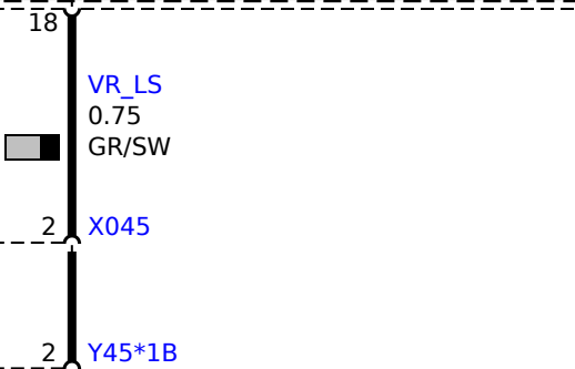
Y45 Valve coil, front right
