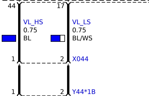
Y44 Valve coil, front left
