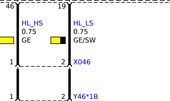
Y46 Valve coil, rear left
