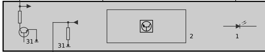
A60 Electrochromic interior rear view mirror 1) LED antitheft alarm system 2) High beam assistant sensor and control
