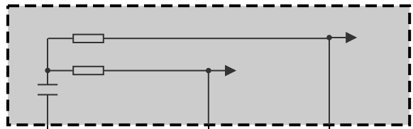
R11 CAN terminator 11
