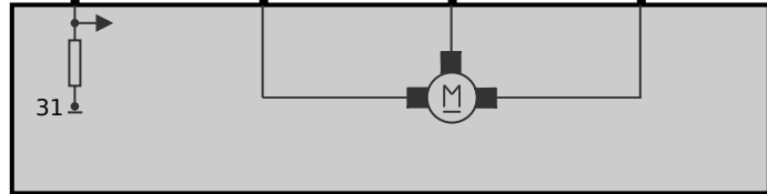
M14 Electric fuel pump
