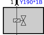
Y6538 Quantity control valve
