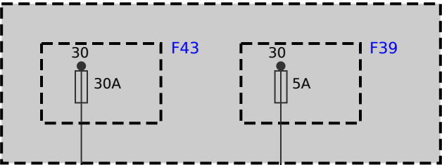
Z7 Front power distribution box
