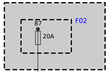
Z42 Power distribution box
