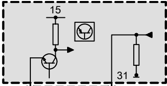
A12 Multiple restraint system control unit
