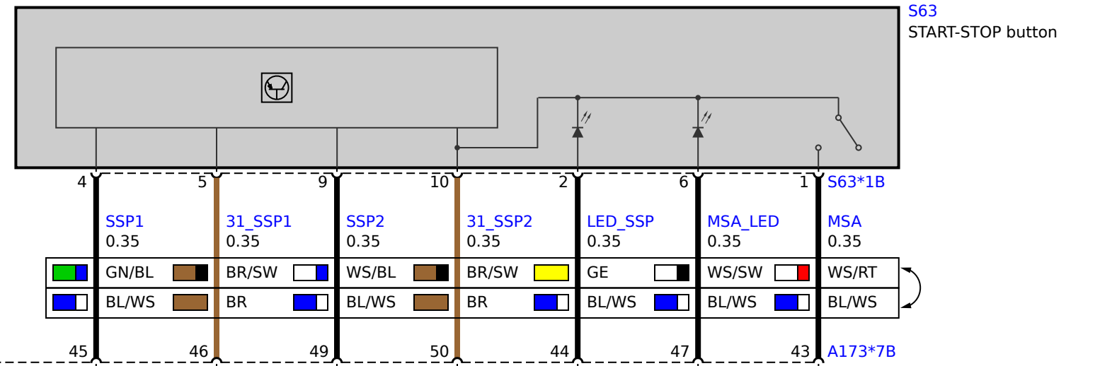
A173 Front Electronic Module
