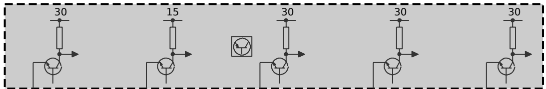
A14286 Function control centre, roof
