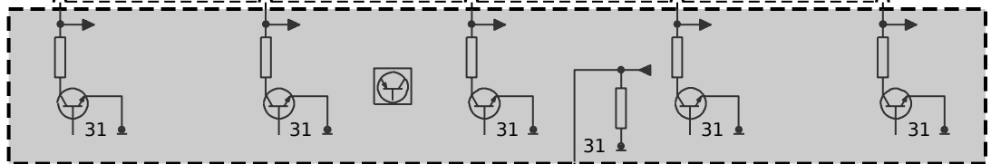
A22 Electrochromic interior rear-view mirror
