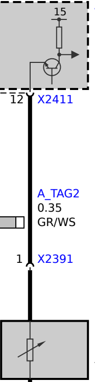
B315 Exhaust temperature sensor upstream of diesel particulate filter
