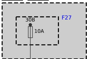
Z7 Front power distribution box
