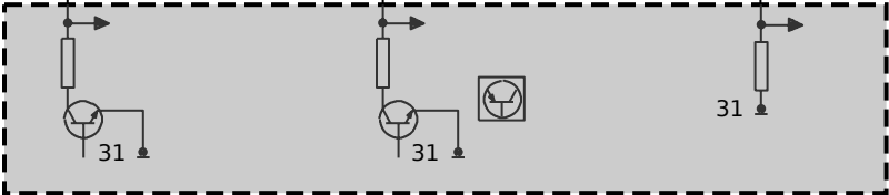
A2249 Digital diesel electronics control unit
