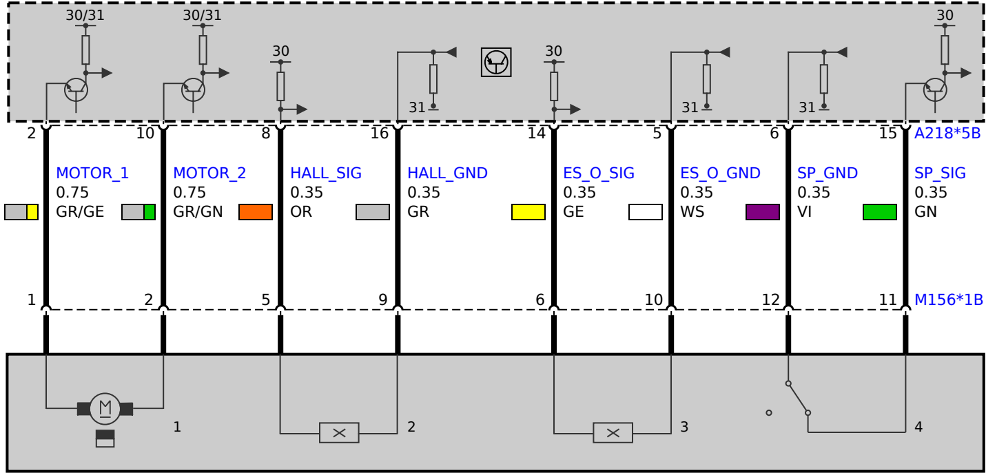
A218a Tailgate function module
