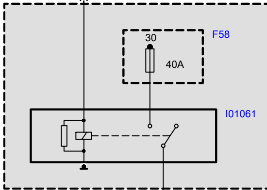
A46 Fuse holder, rear
