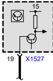
A11a Heating/air conditioning system
