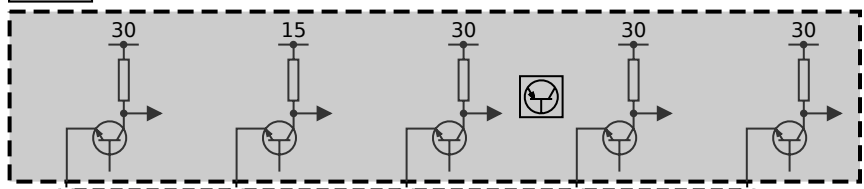
A14286 Function control centre, roof
