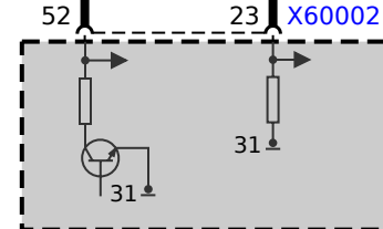
A6000 DME control unit
