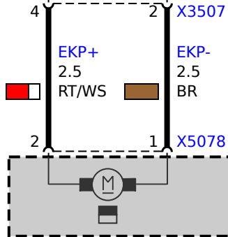
M2 Electric fuel pump
