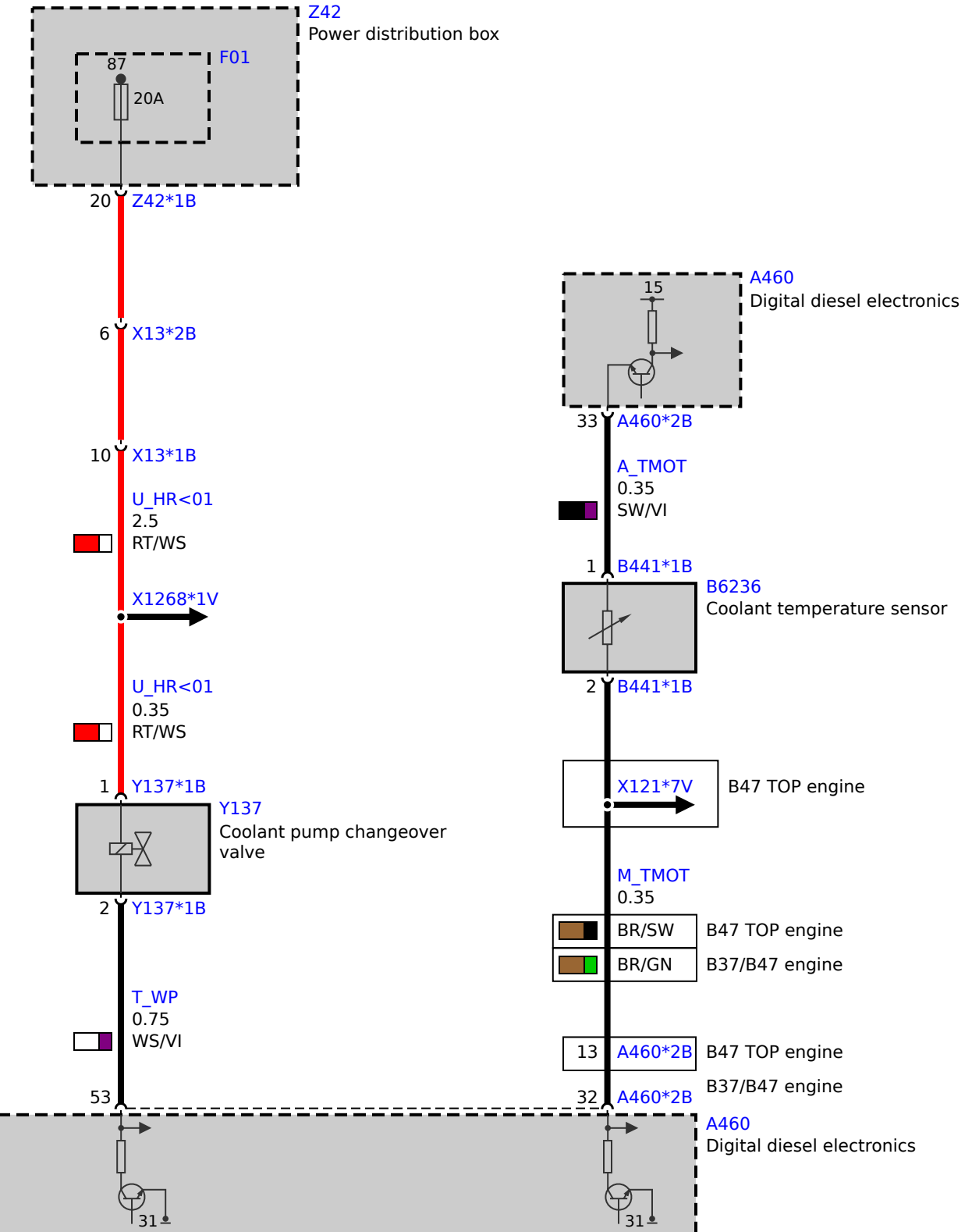
B37 engine
