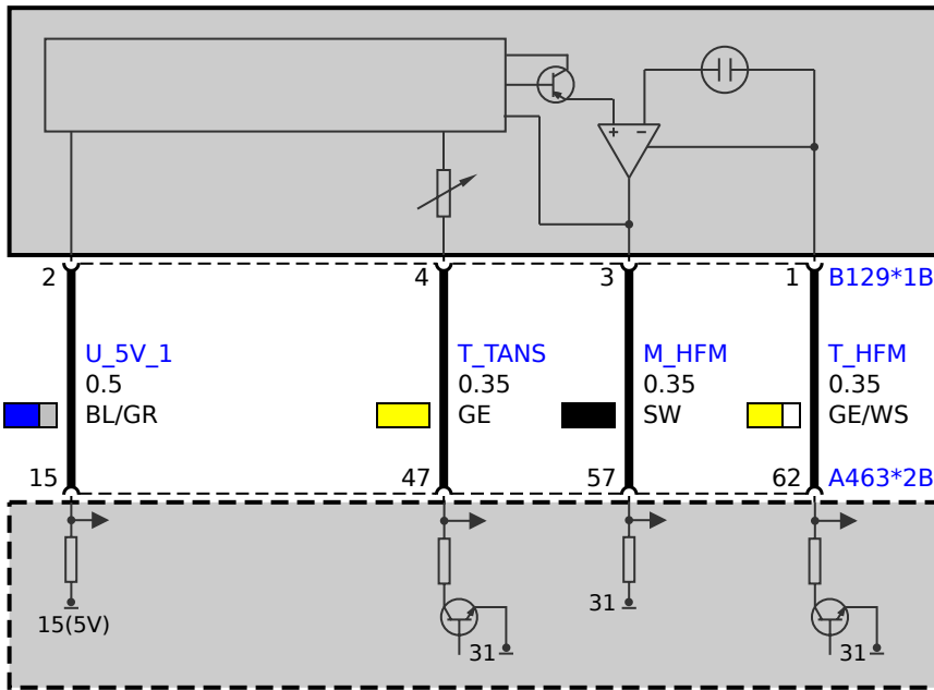
B129 Hot-film air mass meter
