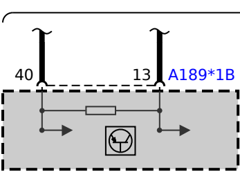
A189 Electronic Damper Control
