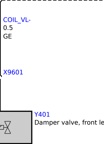
Y401 Damper valve, front left Y402 Damper valve, front right Y403 Damper valve, rear left Y404 Damper valve, rear right
