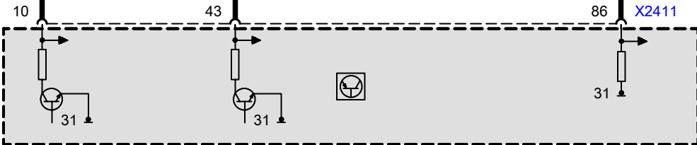
A2249 Digital diesel electronics control unit
