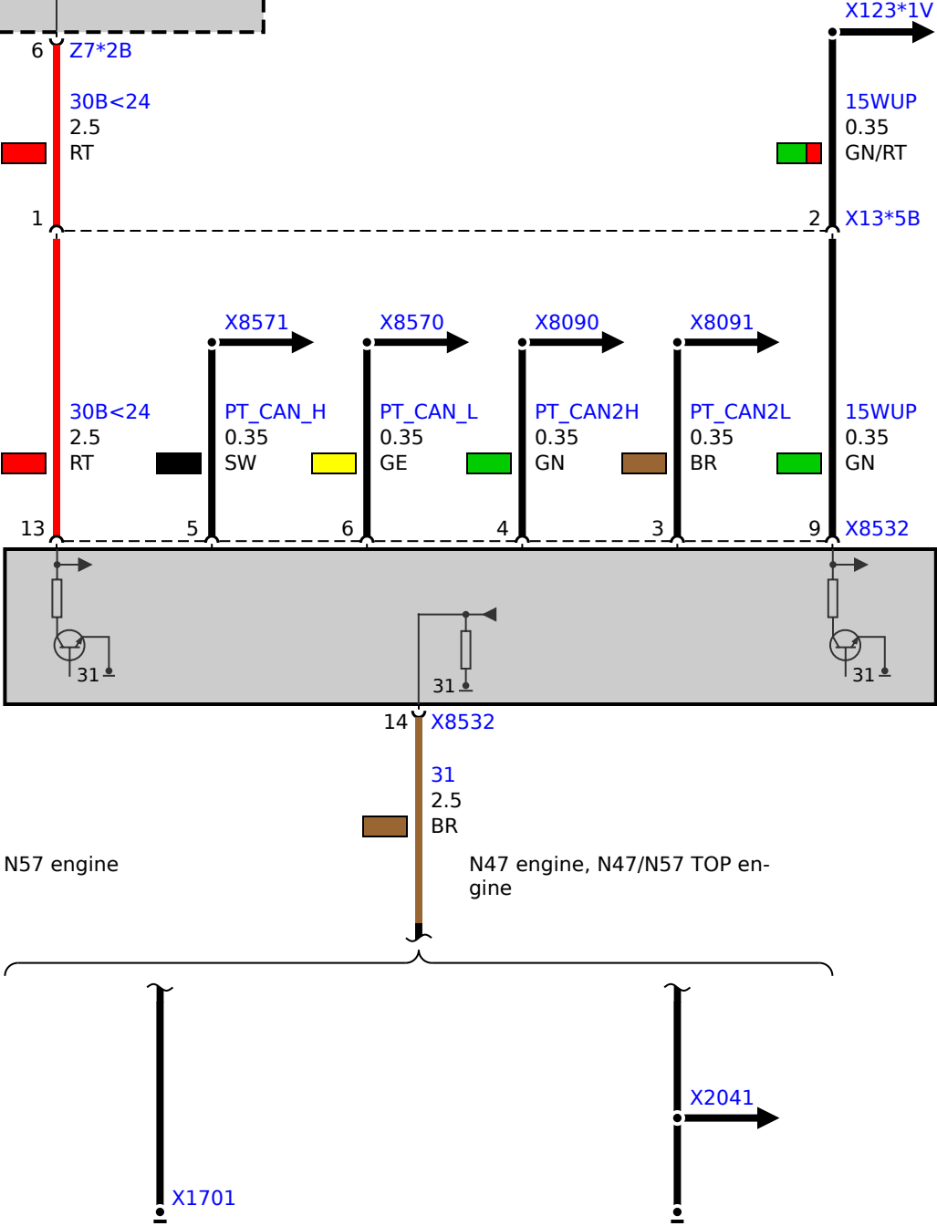
Y21 Electronic transmission control
