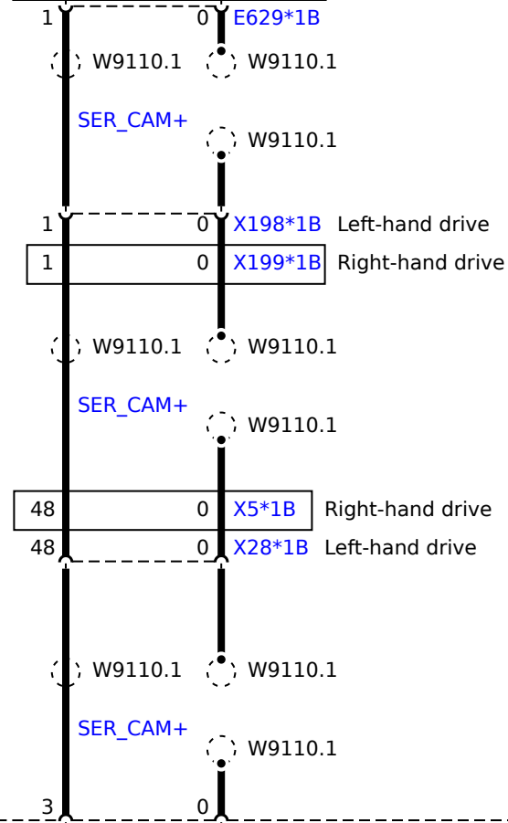
E629 Autonomous Parking Camera, left
