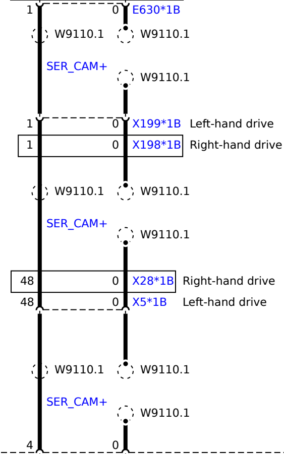
E630 Autonomous Parking Camera, right
