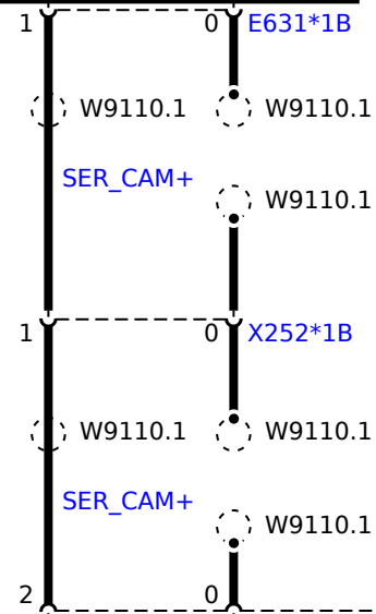
E631 Autonomous Parking Camera, front
