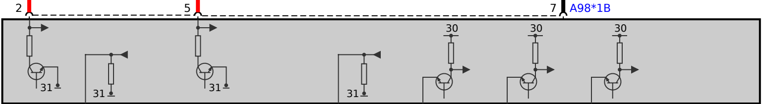
A98a Electric fuel pump control electronics
