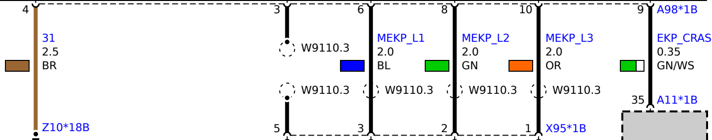
A11 Crash safety module
