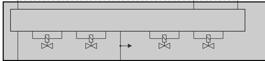
Y74 Valve block, lumbar support, front passenger
