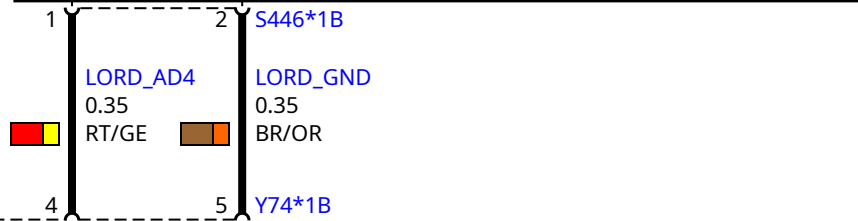
Y74 Valve block, lumbar support, front passenger
